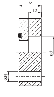
Socket weld
